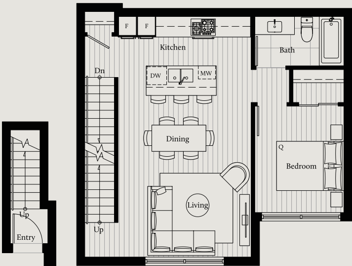
Lower
